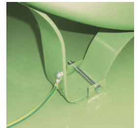
Tank's grounding system
